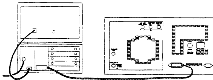
Figure 1-2. HP-IB Connections
